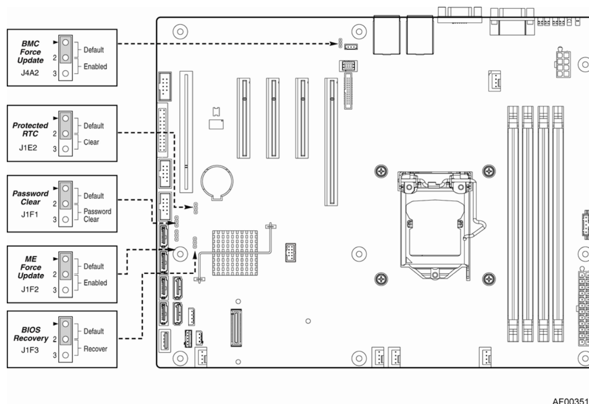
Figure 46. Jumper Blocks (J4A2, J1F1, J1F3, J1F2, and J1E2) on S1200BTL
