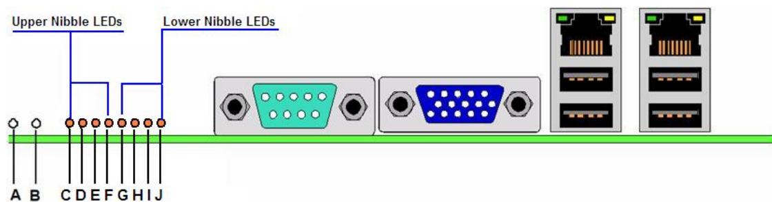
Figure 48. POST Code Diagnostic LED Location
