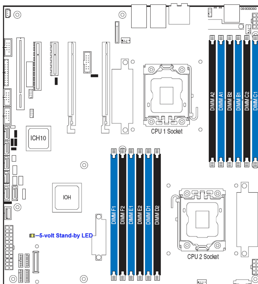
Figure 46. 5V Stand-by Status LED Location
