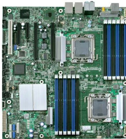
Figure 1. Intel® Workstation Board S5520SC Layout
