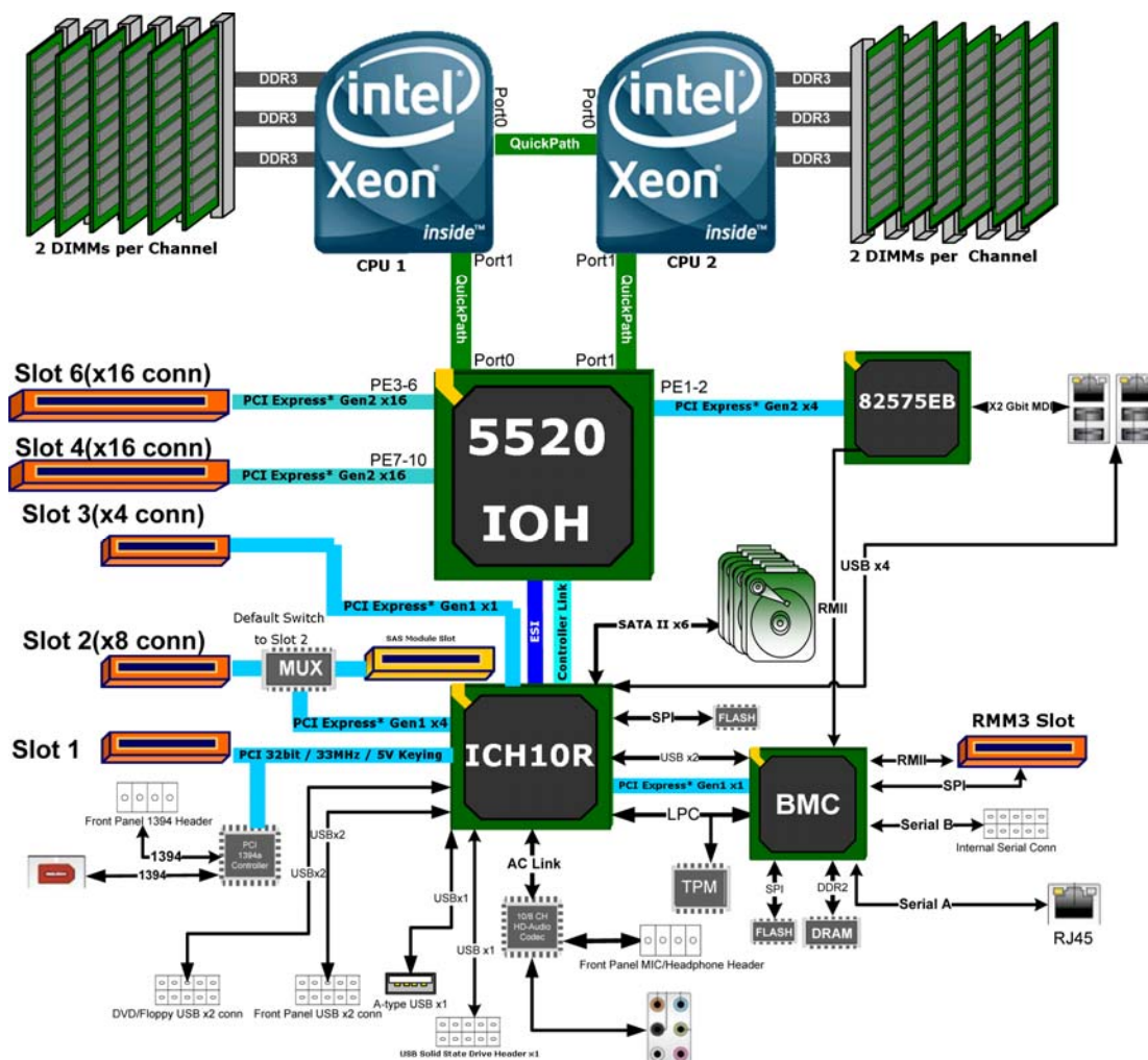
Figure 13. Intel® Workstation Board S5520SC Functional Block Diagram
