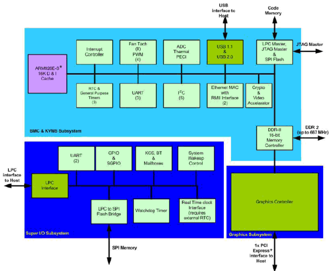
Figure 17. Integrated BMC Hardware
