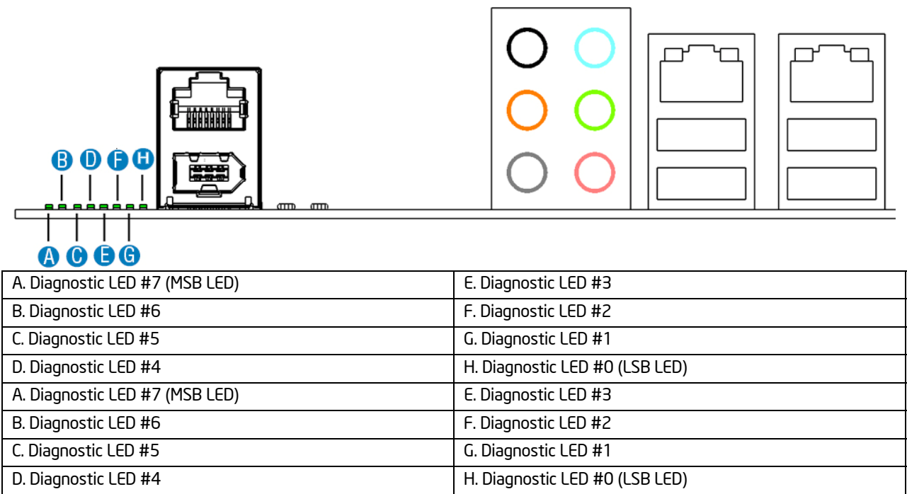
Figure 50. POST Code Diagnostic LED Locations
