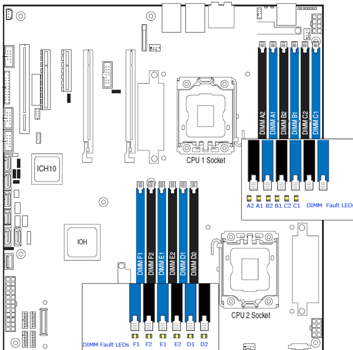
Figure 49. DIMM Fault LEDs Location
