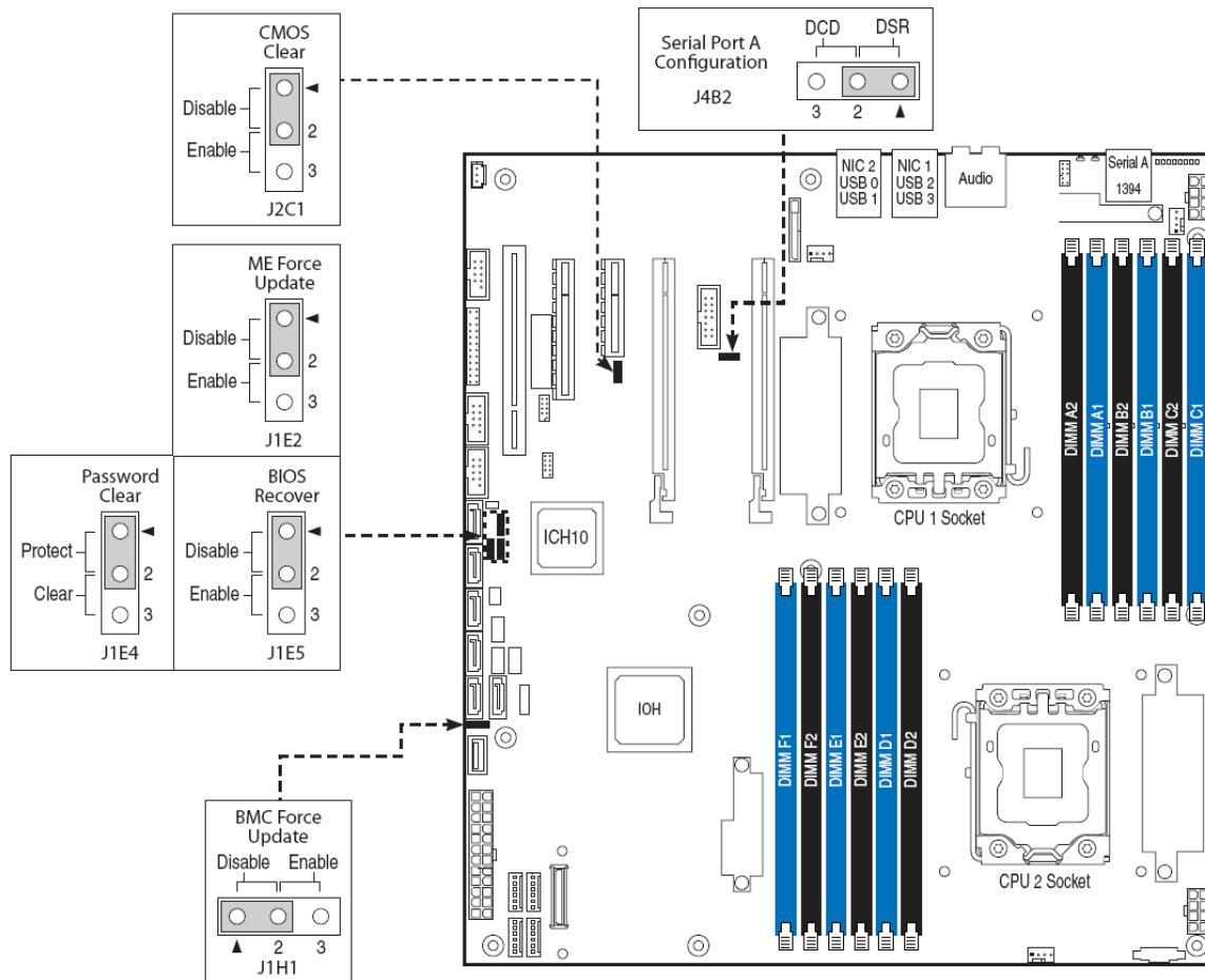
Figure 45. Jumper Blocks
