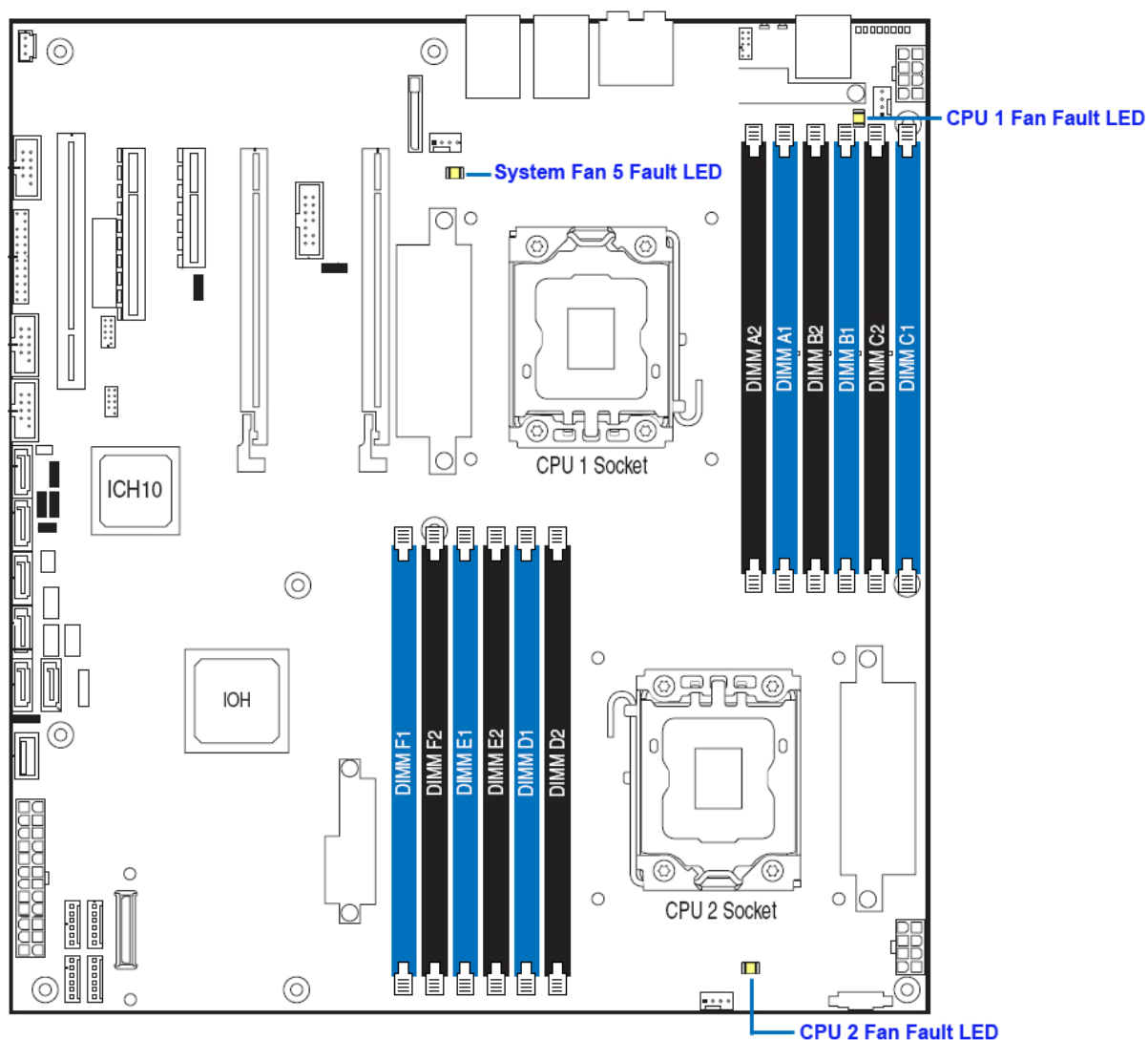
Figure 47. Fan Fault LED Locations
